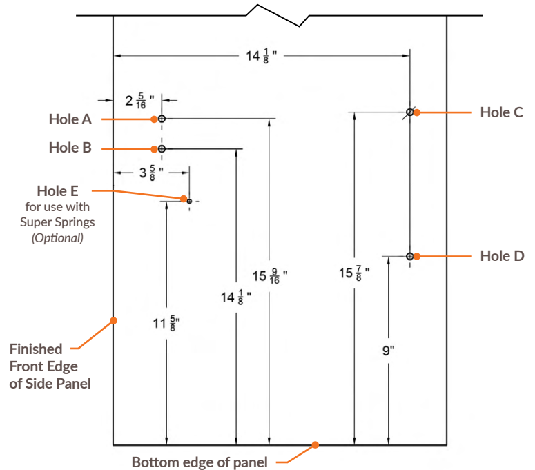
Figure 8: Inside of Left Side Panel
