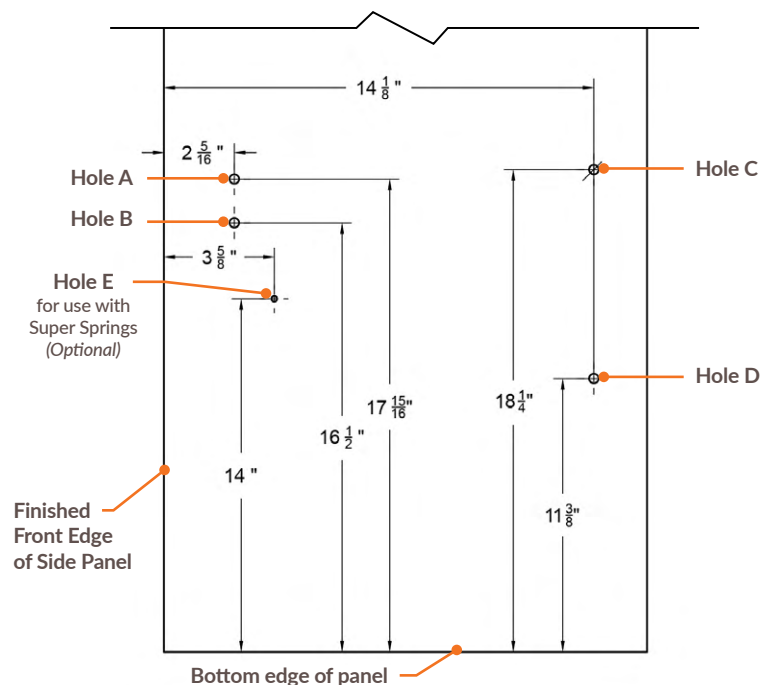
Figure 9: Inside of Left Side Panel
